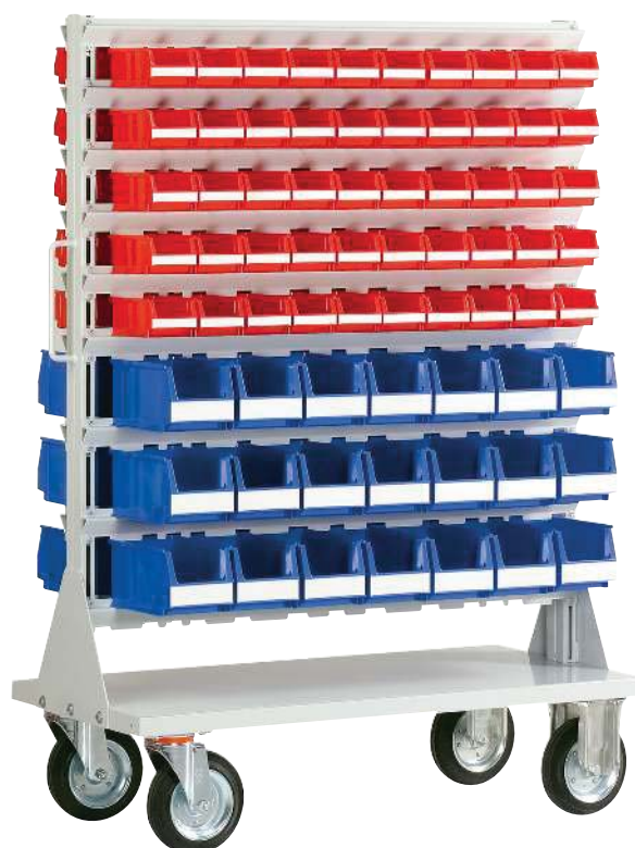
SB M 142 Hanging rack BM 2sided Ext. dimensions: 1150x500x1570 mm with 18 hanging rails
