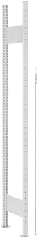
AR 400 Additional frame SD Ext. dimensions: 1000x400x2000 mm
